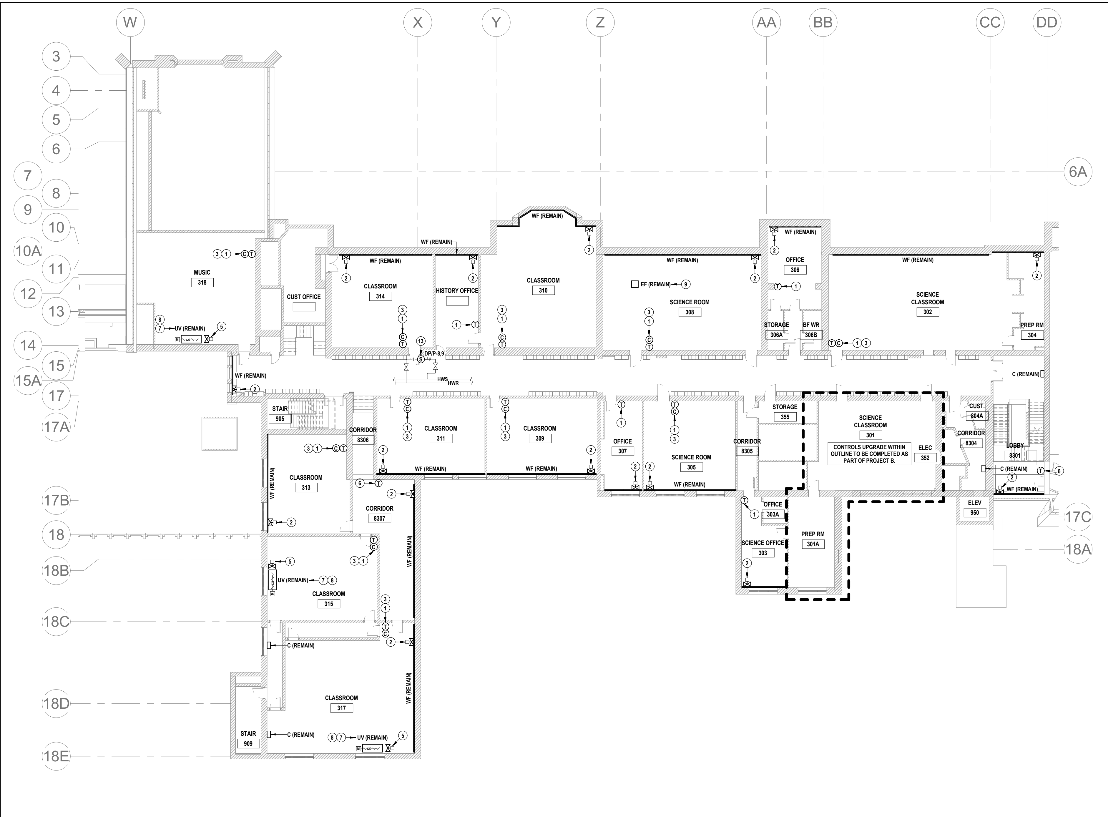
2 HVAC CONTROLS UPGRADES & BUILDING AUTOMATION SYSTEM EXPANSION (THIRD FLOOR EAST) - 1906/1923 ADDITION M5.3 SCALE: 1:200
