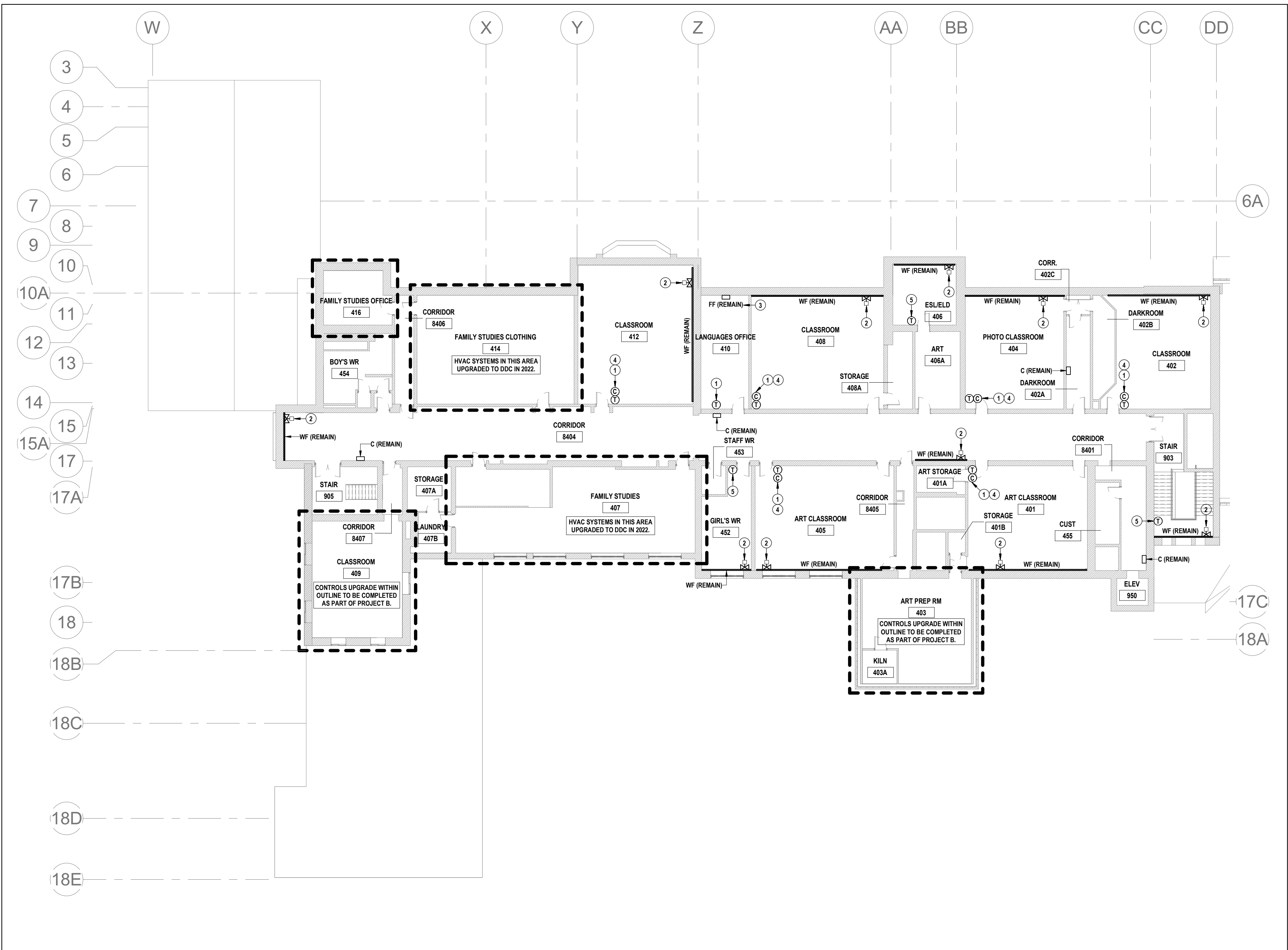
1 HVAC CONTROLS UPGRADES & BUILDING AUTOMATION SYSTEM EXPANSION (FOURTH FLOOR EAST) - 1906/1923 ADDITION M5.4 SCALE: 1/200
