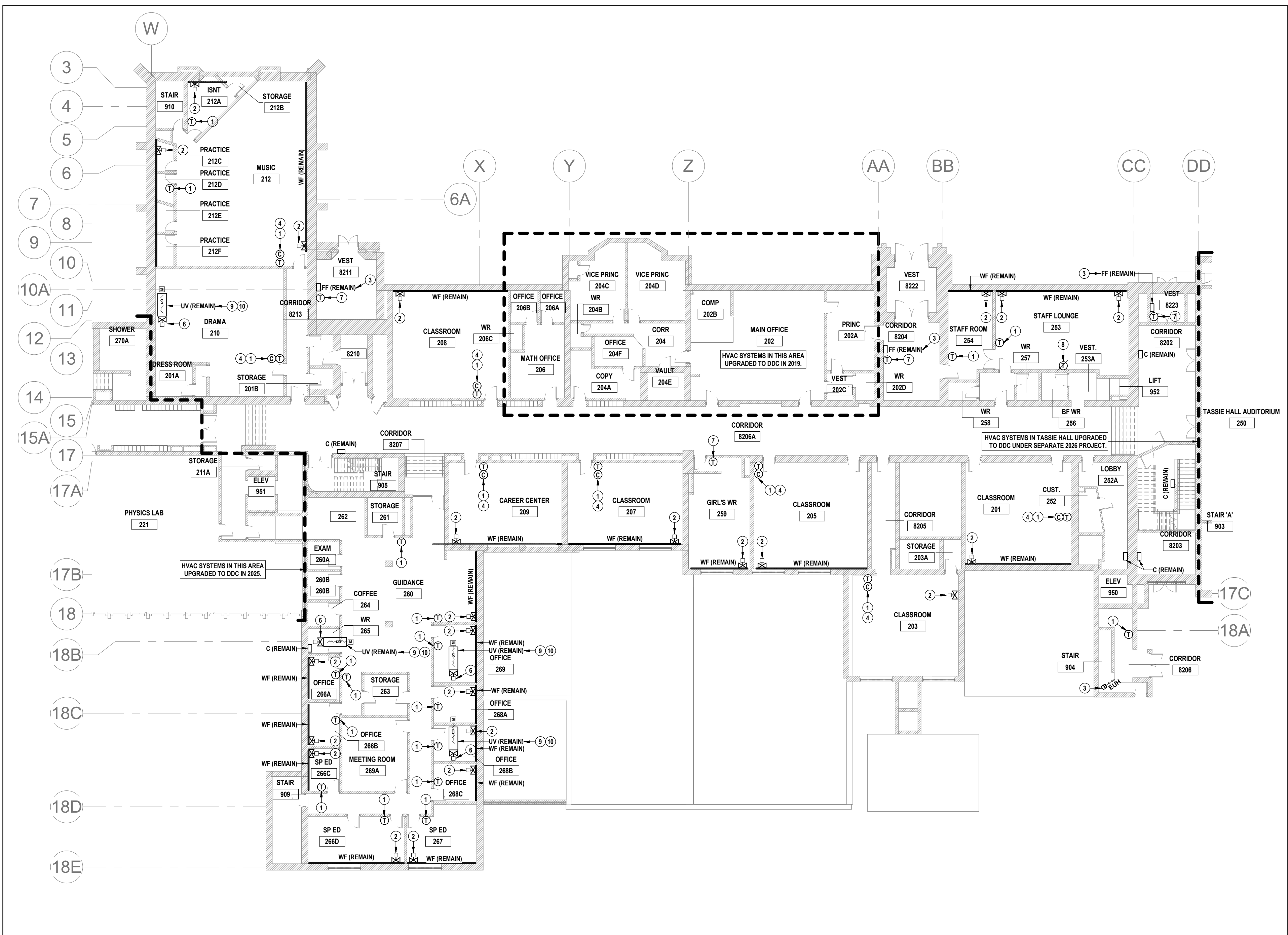
2 HVAC CONTROLS UPGRADES & BUILDING AUTOMATION SYSTEM EXPANSION (SECOND FLOOR EAST) - 1906/1923 ADDITION MS.2 SCALE: 1 : 200
