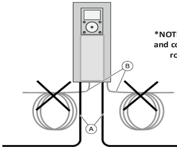
A – MOTOR CABLES B – FIELDBUS CABLES
