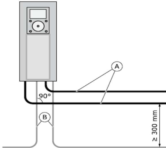
A – MOTOR CABLES B – FIELDBUS CABLES
