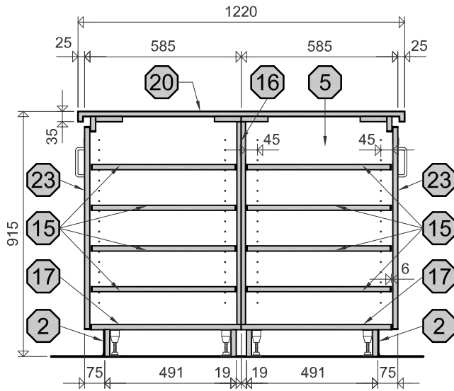
1 TYPICAL MILLWORK SECTION CUTTING TABLE
