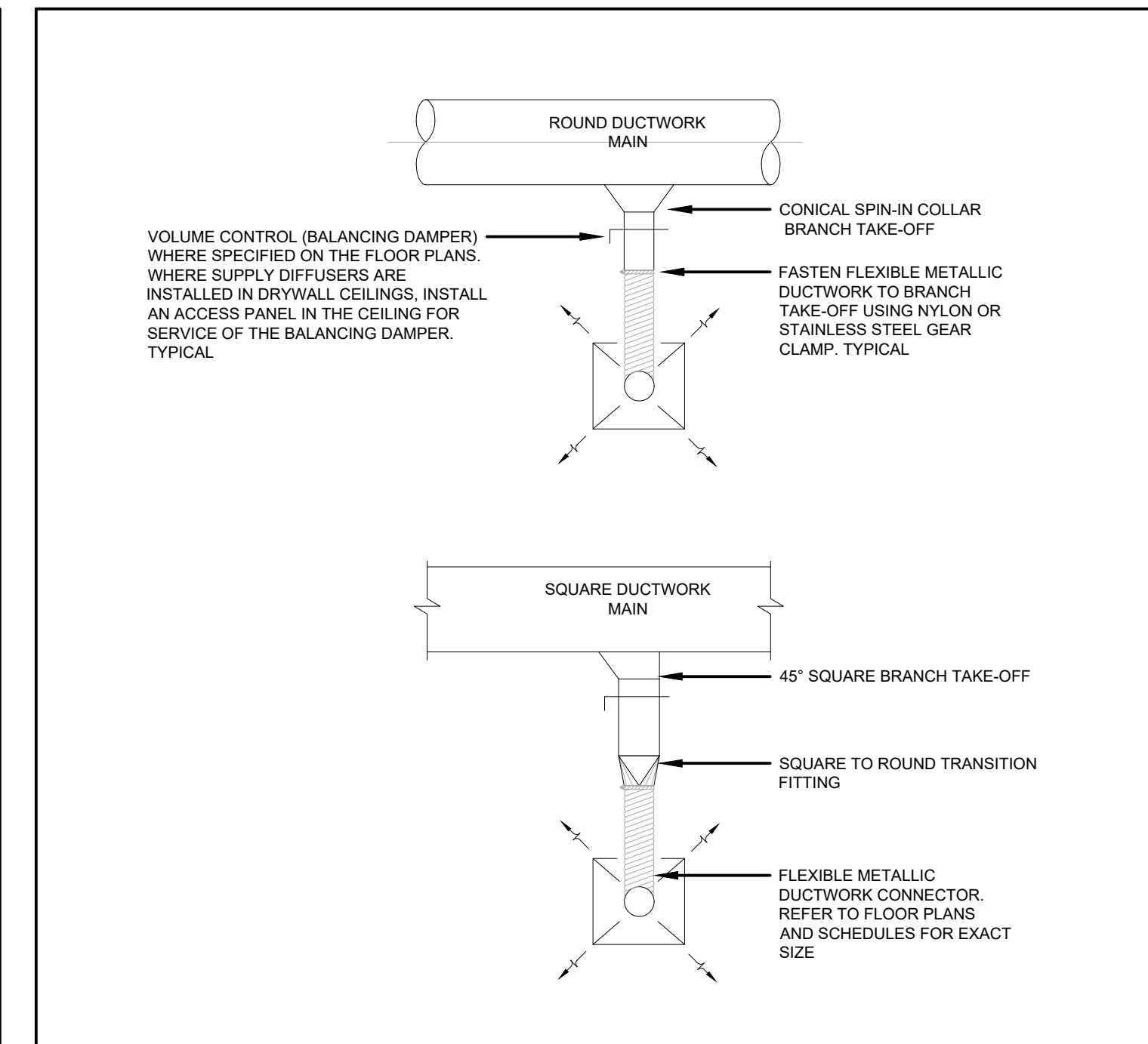
4 FLEXIBLE METALLIC DUCTWORK CONNECTION NOT TO SCALE
