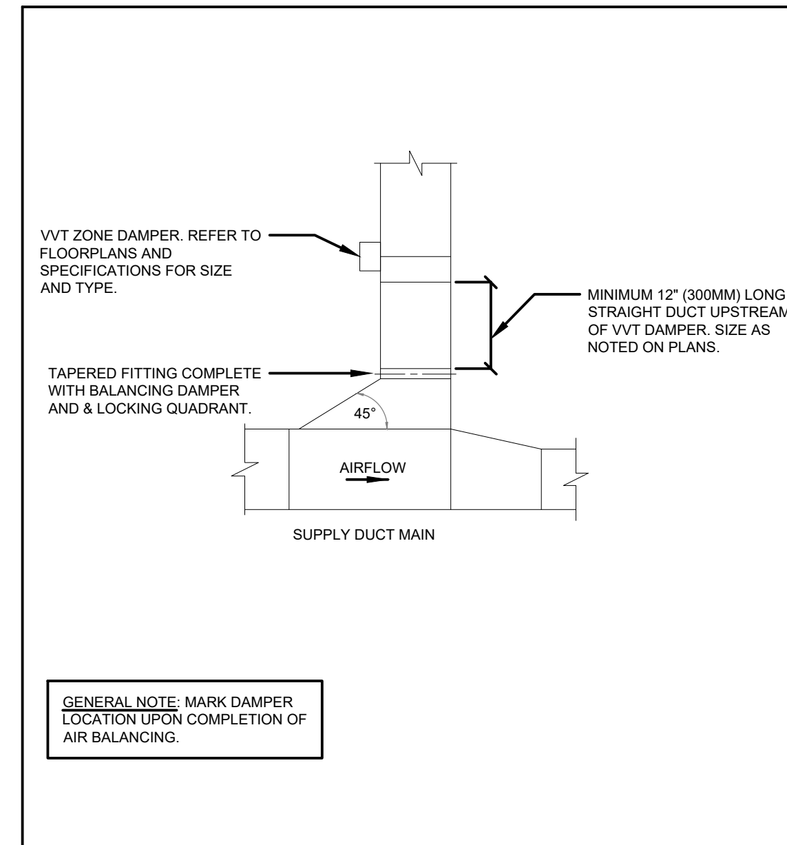
9 TYPICAL VVT DAMPER INSTALLATION NOT TO SCALE
