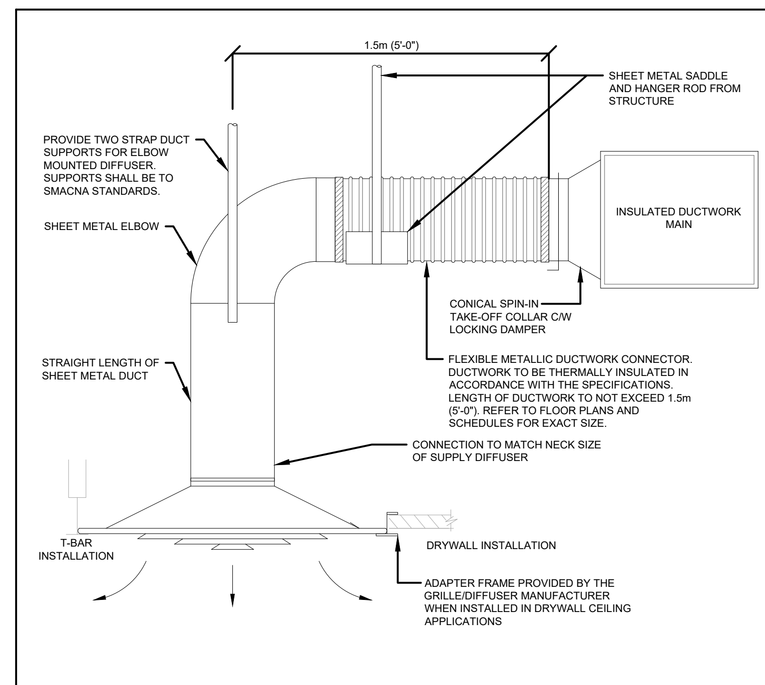
3 FLEXIBLE METALLIC DUCTWORK NOT TO SCALE
