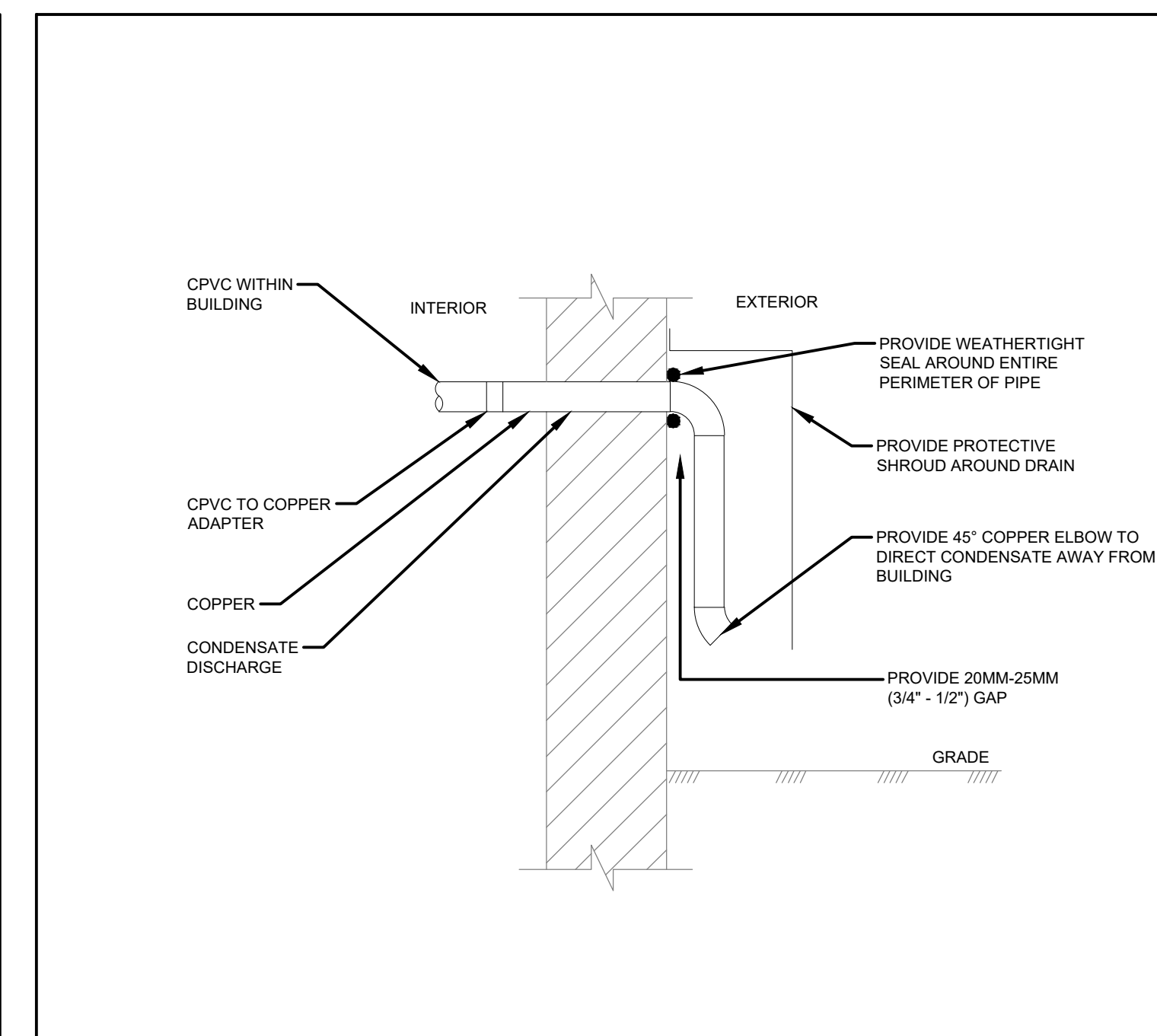
1 20 05 05.08 EXTERIOR CONDENSATE PIPING DISCHARGE DETAIL NOT TO SCALE
