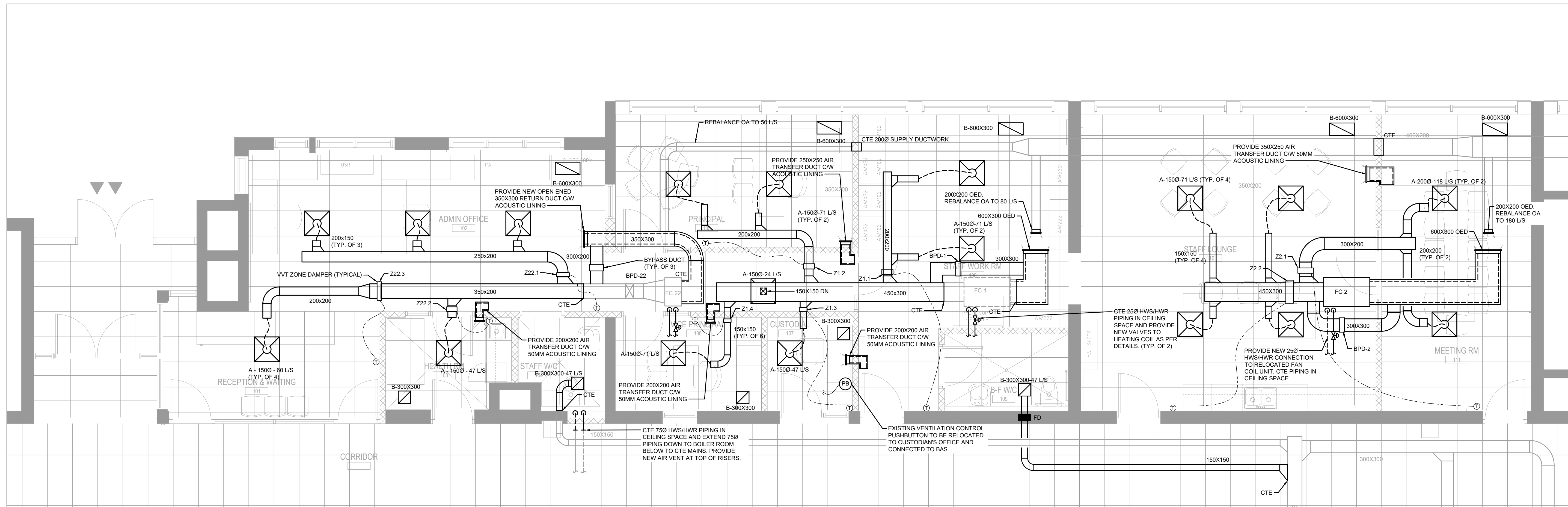
2 HVAC - NEW WORK PLAN SCALE: 1:50
