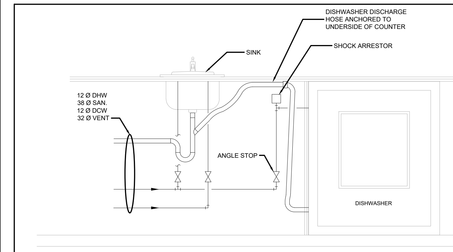
7 DISHWASHER PLUMBING CONNECTION NOT TO SCALE
