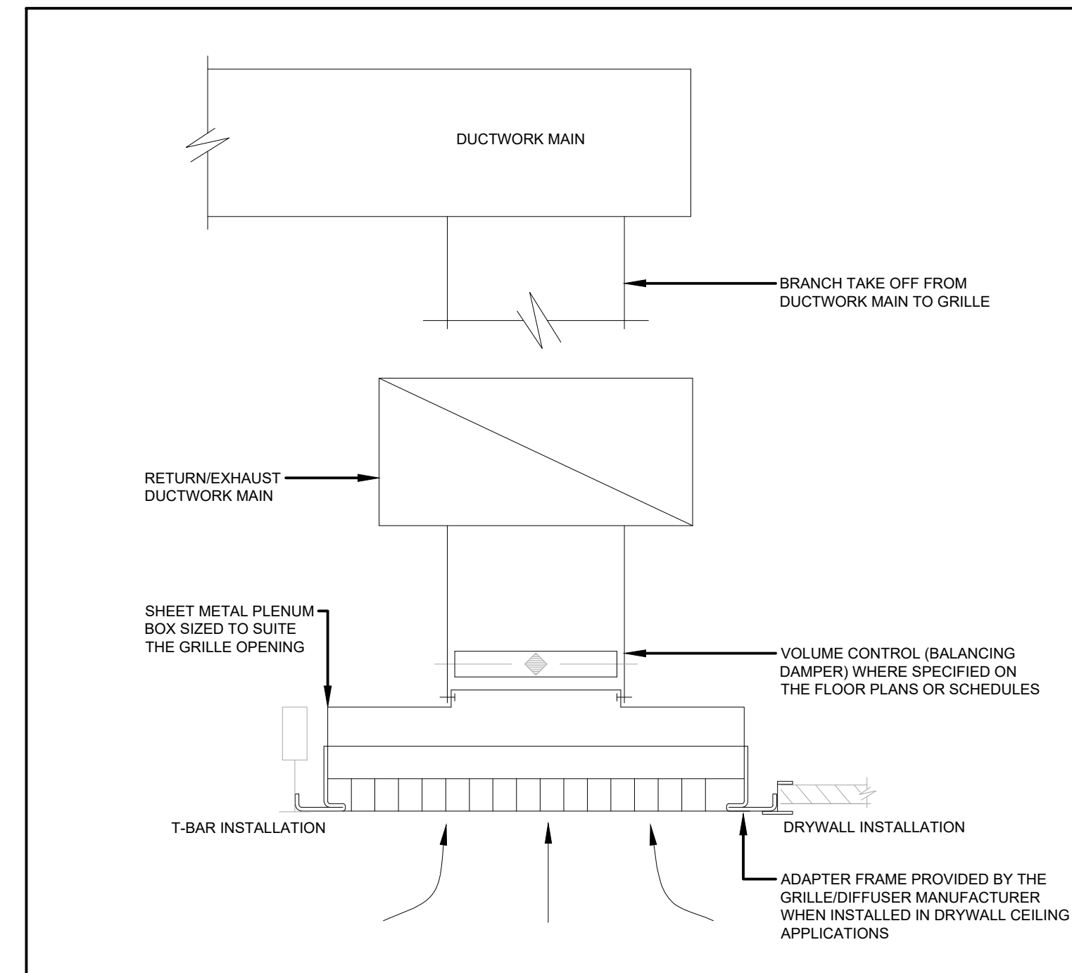
5 CEILING RETURN GRILLE MOUNTING ARRANGEMENT NOT TO SCALE
