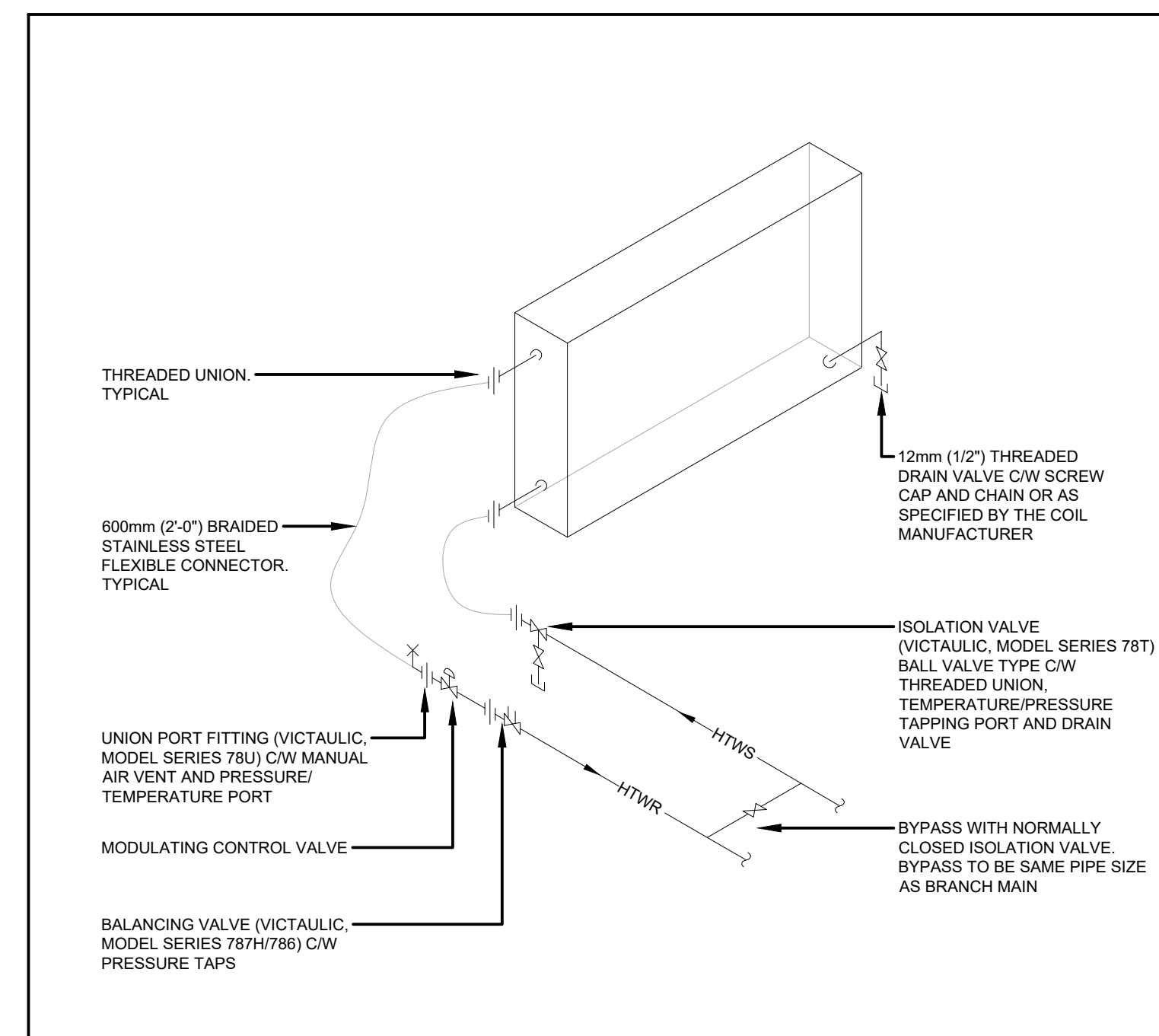
2 DUCT MOUNTED HYDRONIC HEATING COIL NOT TO SCALE
