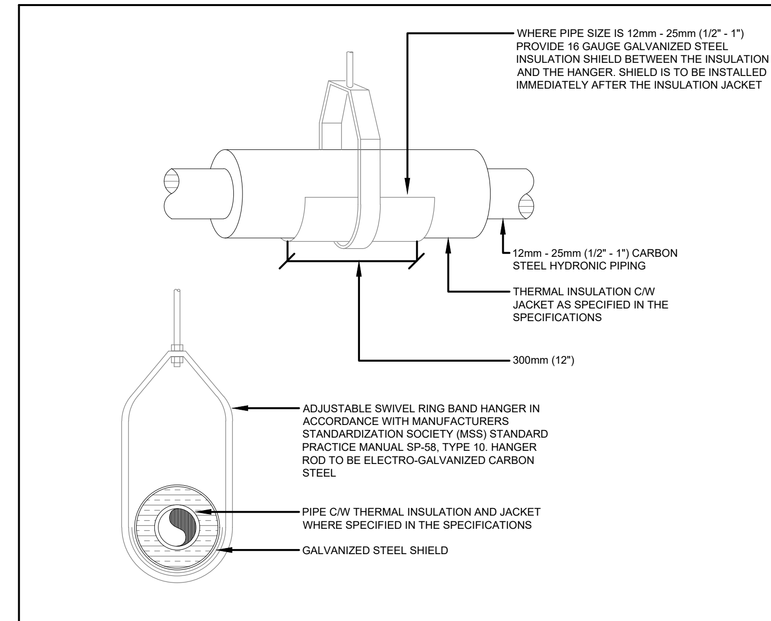
8 PIPING HANGERS AND SUPPORTS NOT TO SCALE
