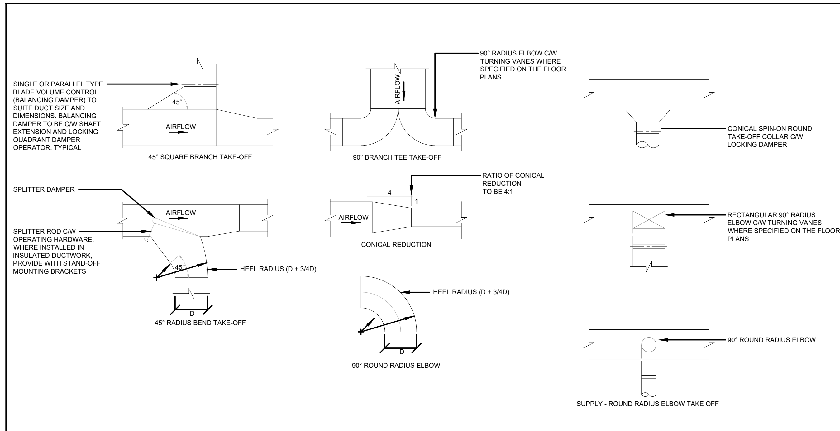
6 DUCTWORK FITTING AND TAKE-OFFS NOT TO SCALE
